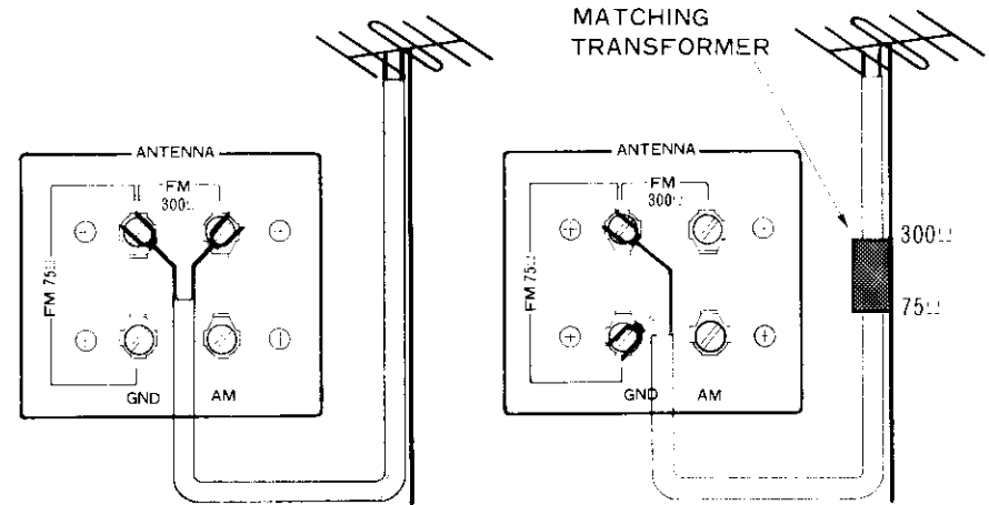
FM ANTENNA CONNECTION
