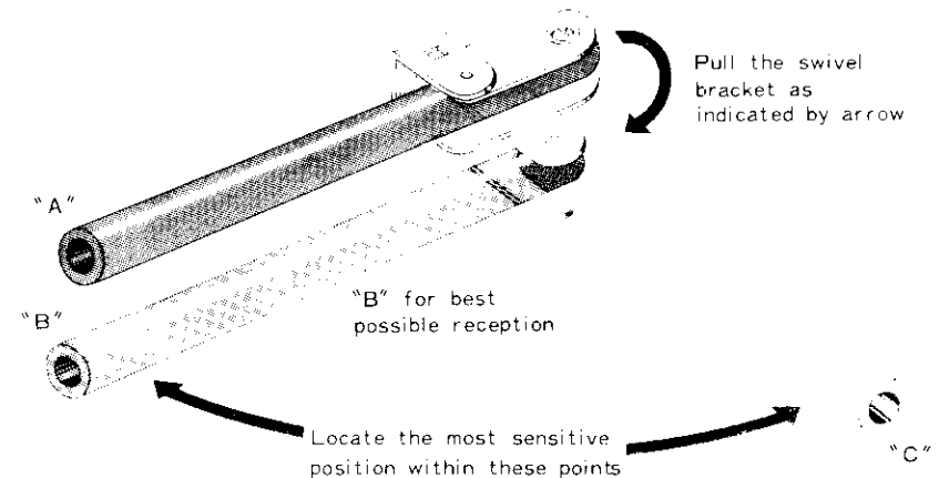
AM ANTENNA SETTING
